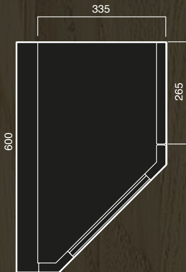
Angled base
